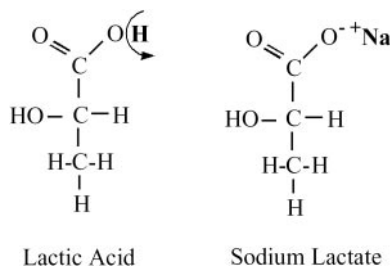
Fig. 1. Chemical structures of lactic acid and the sodium salt of lactate. When the proton of the carboxylic acid functional group ( -\text{COOH} ) of lactic acid dissociates ( \text{COO}^- + \text{H}^+ ), a cation ionically interacts with the negatively charged oxygen atom of the carboxyl group, forming the acid salt lactate. In this example, the cation is sodium ( \text{Na}^+ ).
